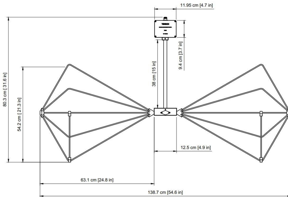
Figure 1: TBMA2 mechanical dimensions
