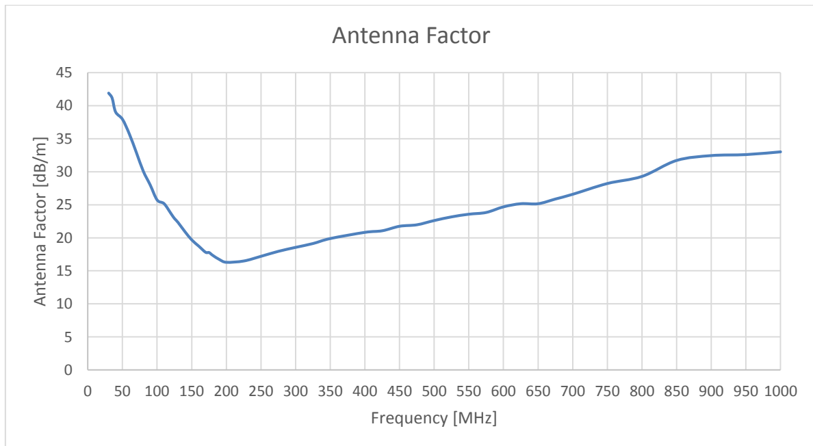
30 MHz...1 GHz , Antenna Factor of TBMA1
