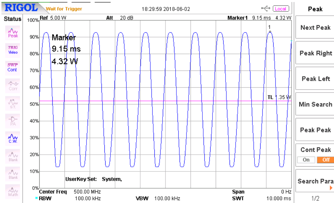
Figure 2 – 1 kHz, 80 % AM envelope, 500 MHz
