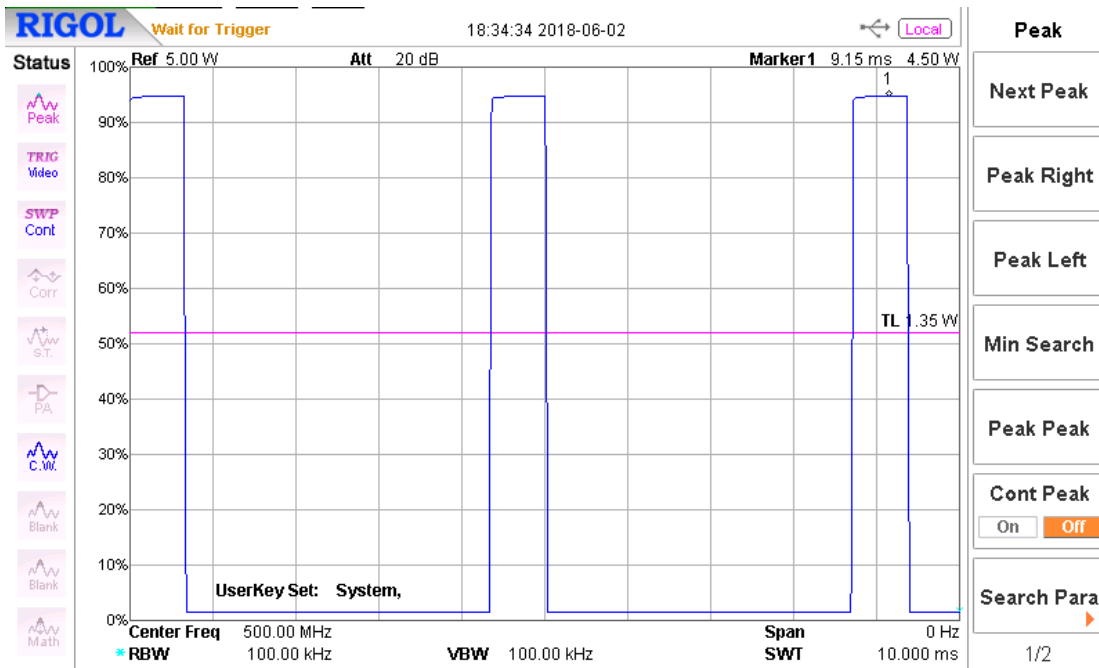
Figure 4 – 217 Hz, 12.5 % PM envelope, 500 MHz
