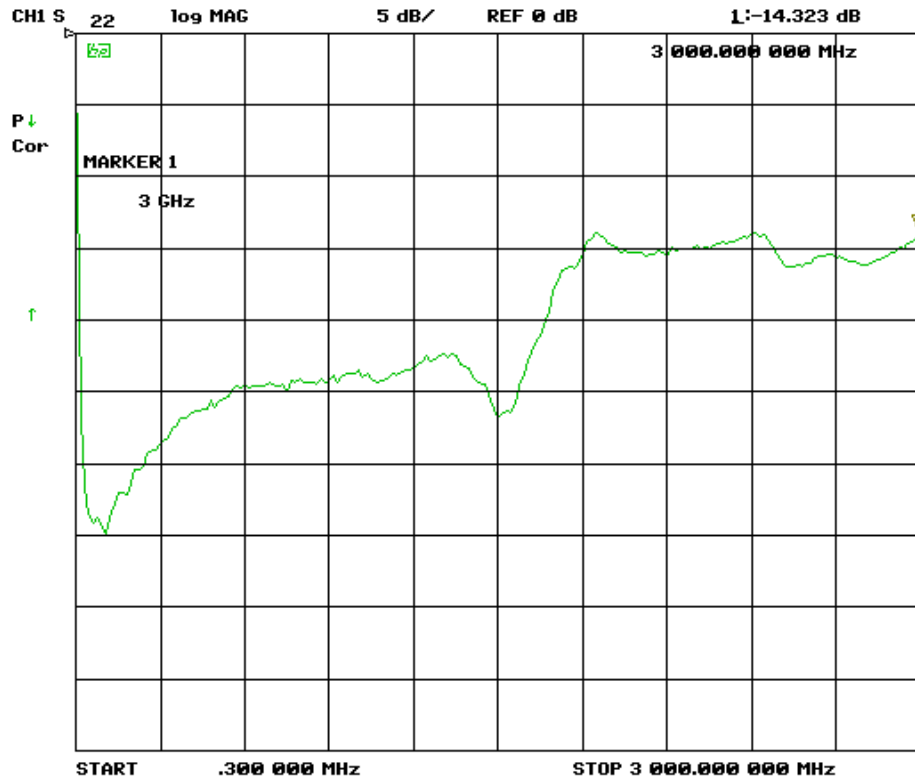
Picture 20 – TBWA2/40dB, output return loss, IS221, 300 kHz – 3 GHz, lin.
