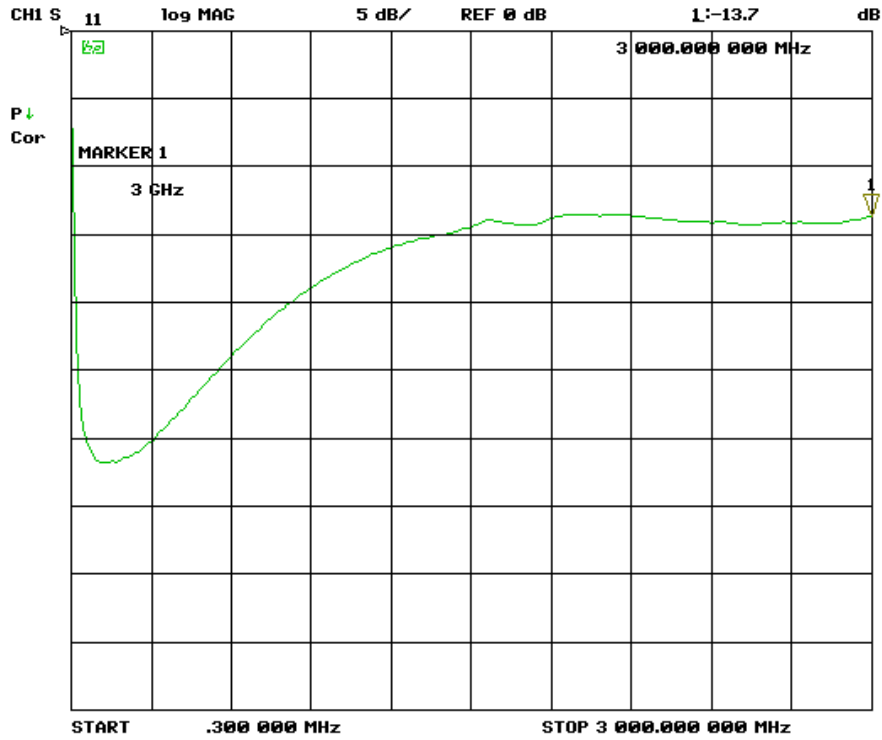
Picture 15 – TBWA2/20dB, input return loss, IS111, 300 kHz – 3 GHz, lin.
