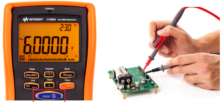
Figure 5. Hold & Export button—one press for three actions: Measure, save it into handheld DMM's memory and send the measurement out via infrared port. Optional U5404A remote switch probe emulates 'Hold & Export' button.
