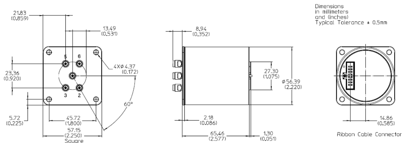
Figure 7. U7104E/N/F mechanical dimension (options 200 and 300) – 16-pin DIP connector
