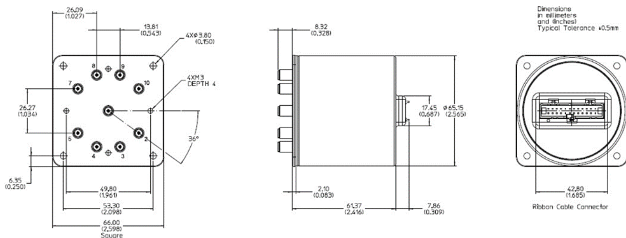
Figure 7. U7108A/B/C mechanical dimension (options 200 and 300) – 24-pin DIP connector
