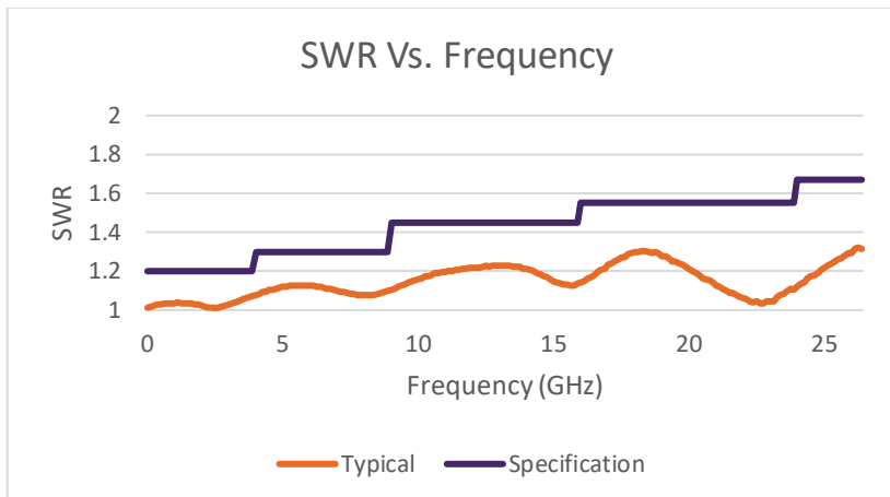
Figure 4. SWR versus frequency typical plot
