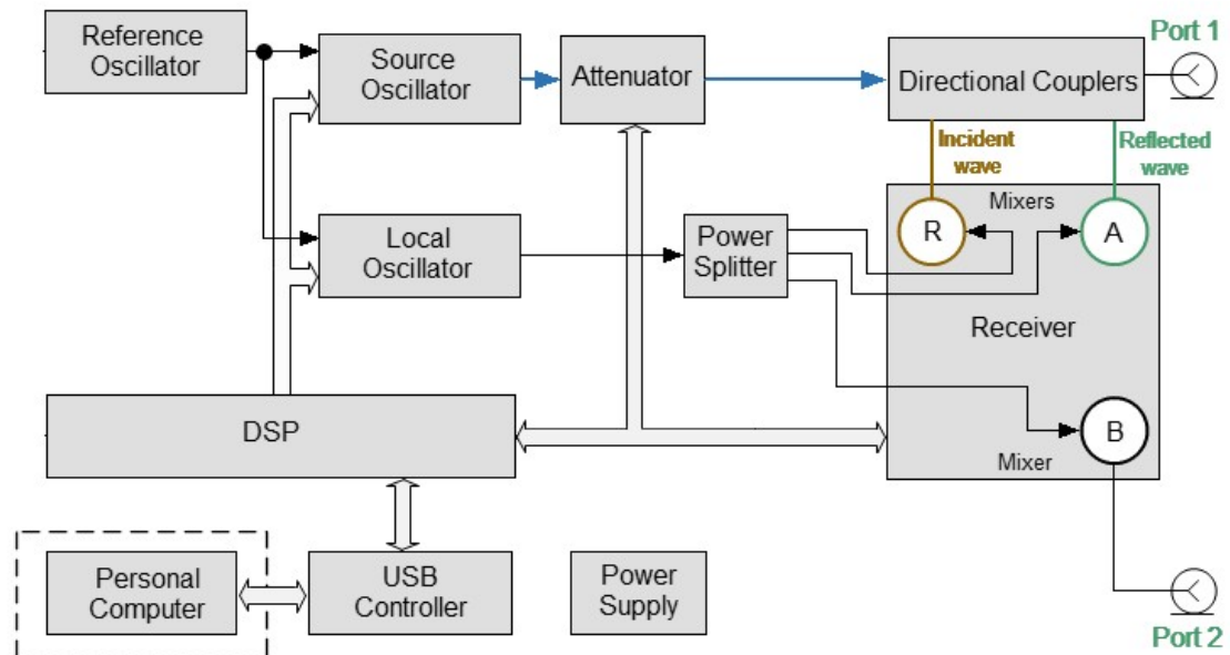
VTR0102 and VTR0302 Block Diagram
