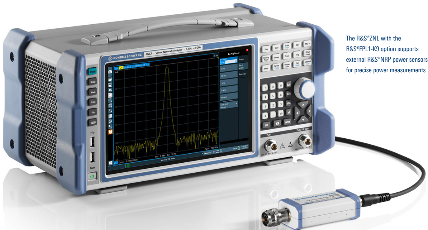
Examples of R&S®NRP power sensors: R&S®NRP8SN and R&S®NRP8S three-path diode power sensors.
