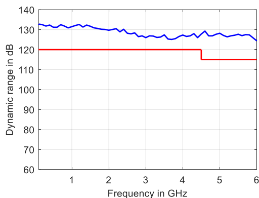
Measured dynamic range in dB versus frequency for the R&S®ZNL3, R&S®ZNL4 and R&S®ZNL6
