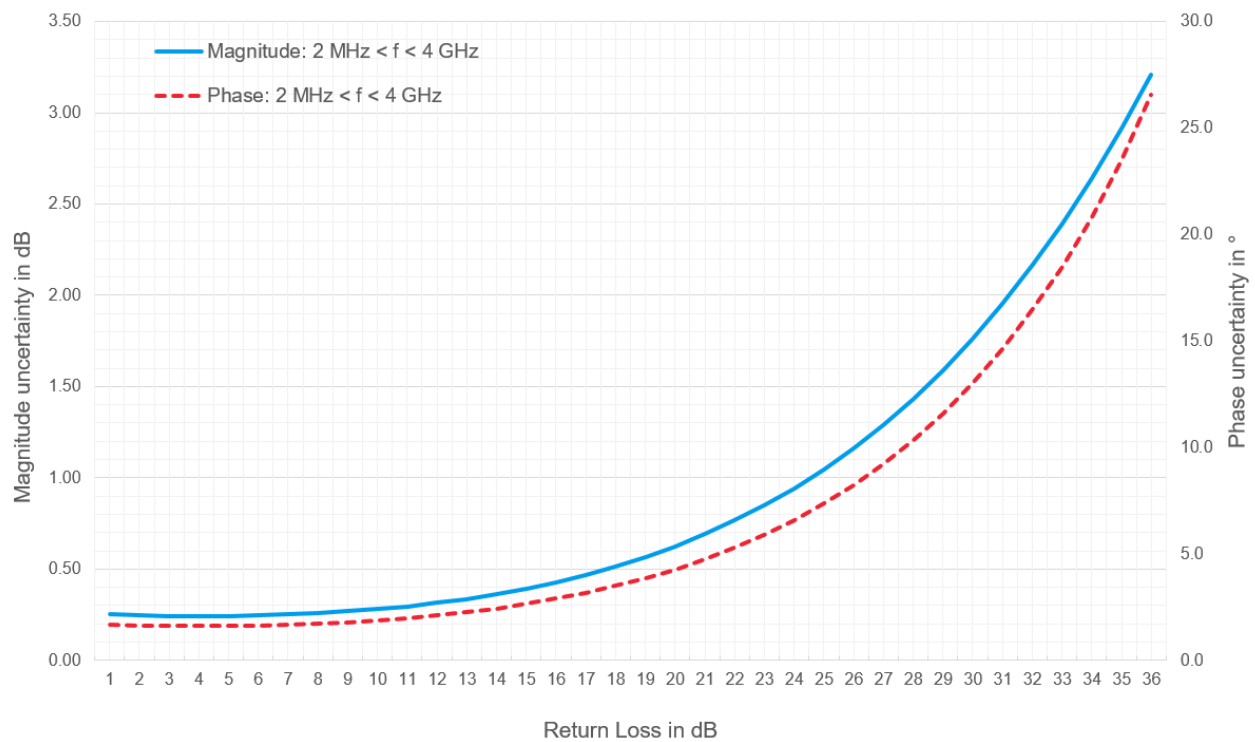
Uncertainty of reflection measurements with R&S®ZN-Z103 Temp: +18 °C to +25 °C, RBW: 10 Hz, Power: -10dBm
